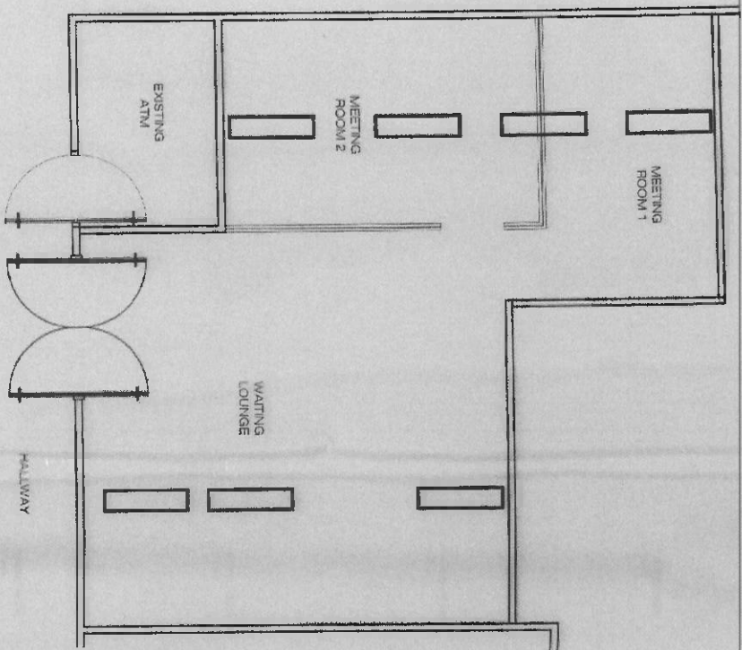
1 EXISTING LIGHTING FIXTURES SCALE: 1:50MTRS
