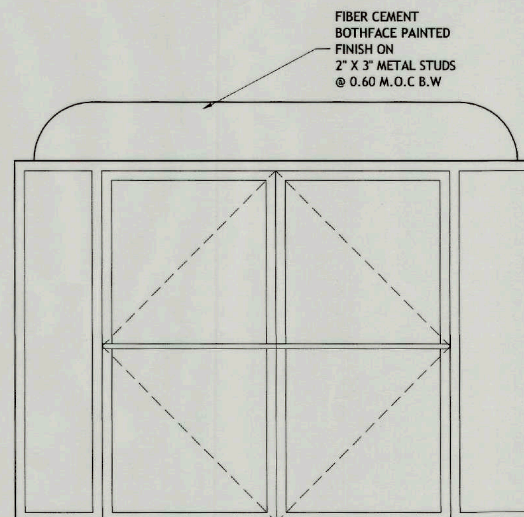
DETAIL OF DOOR
