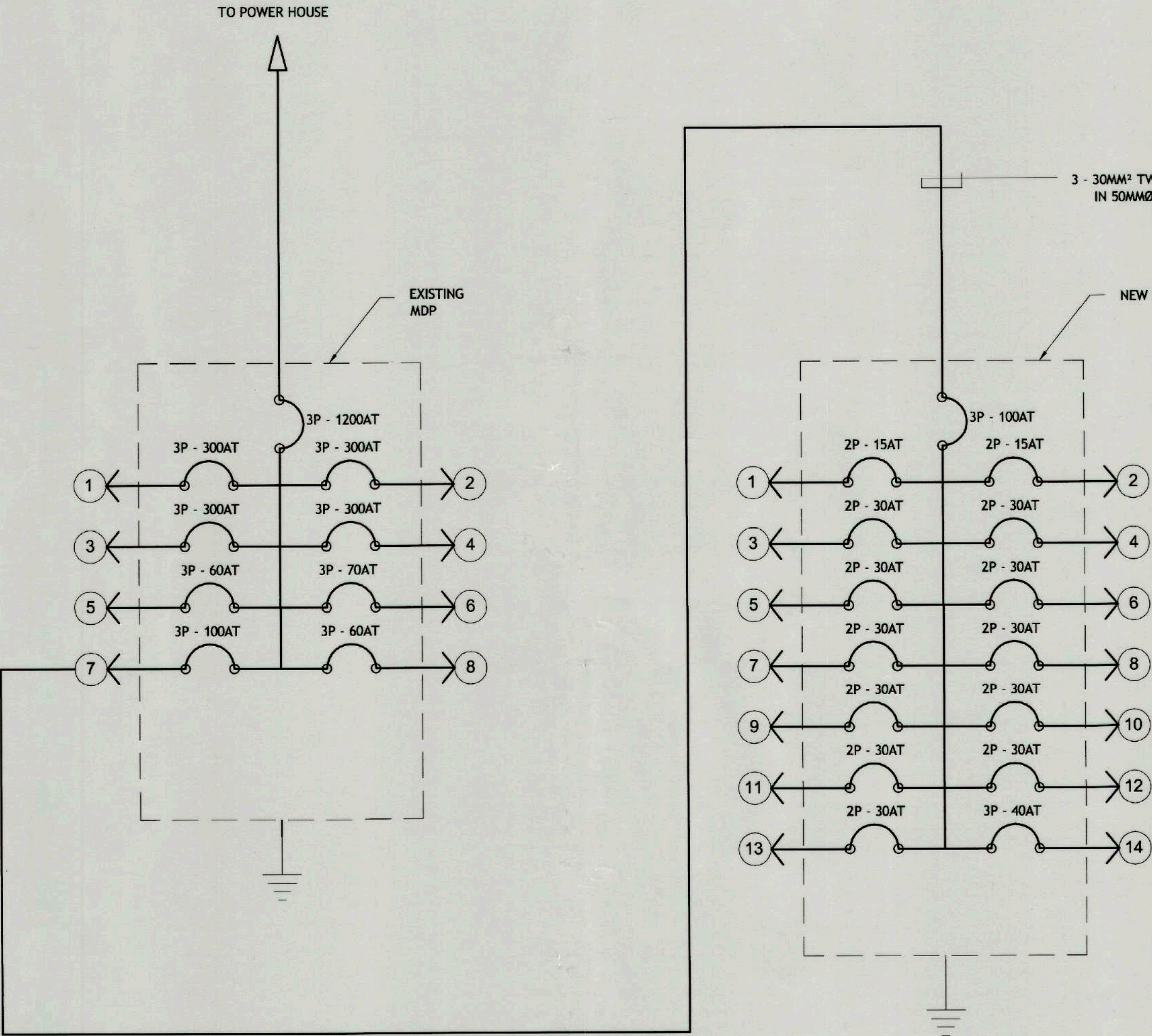
RISER DIAGRAM
