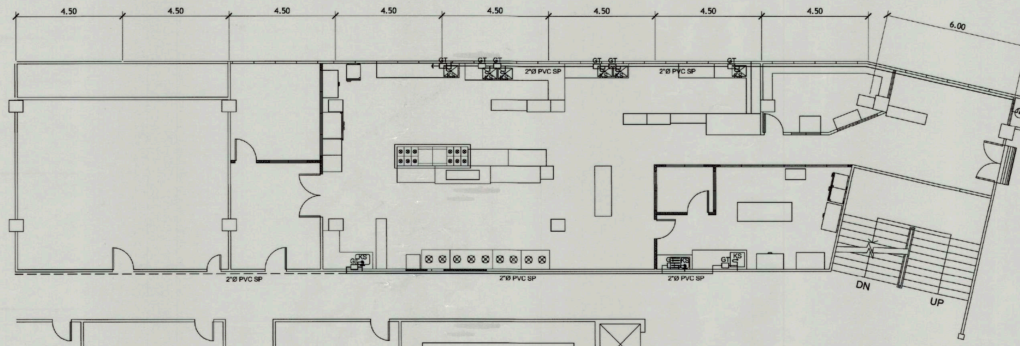
KITCHEN SEWER LINE LAYOUT SCALE 1 : 100 MTS
