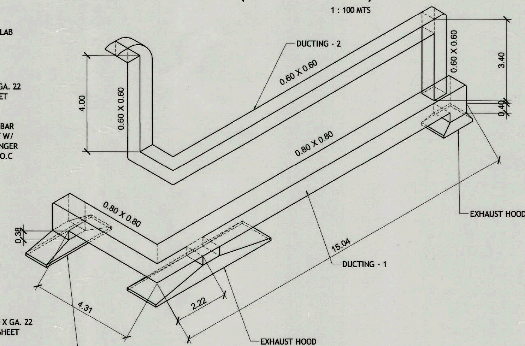
EXHAUST DUCTING ISOMETRIC
