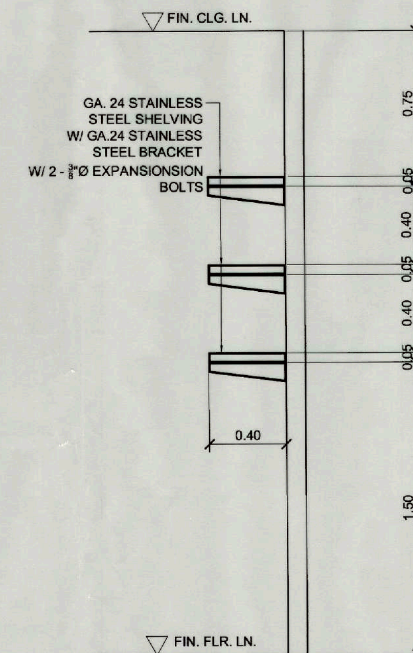
SHELVES DETAIL
