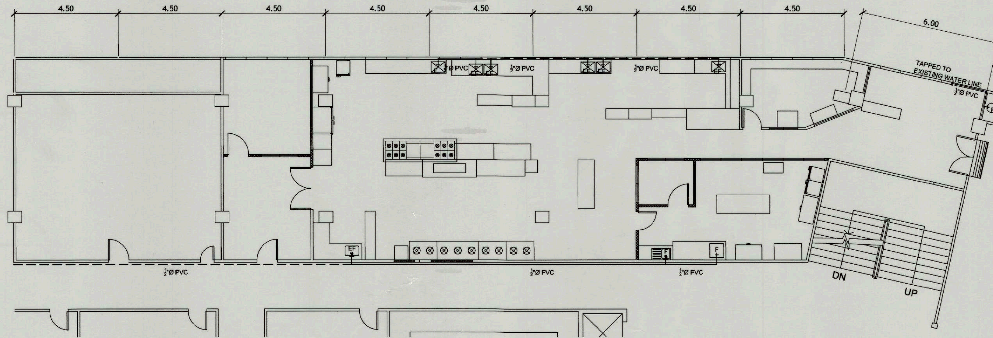
KITCHEN WATER LINE LAYOUT SCALE 1 : 100 MTS
