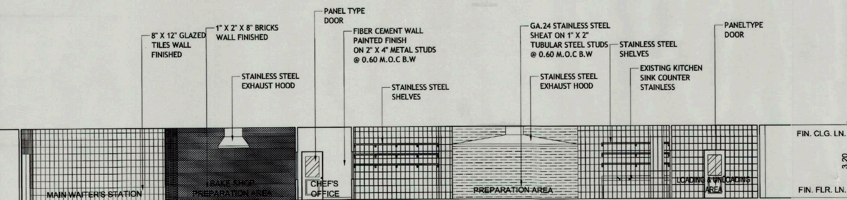
SECTION THRU LINE - B
