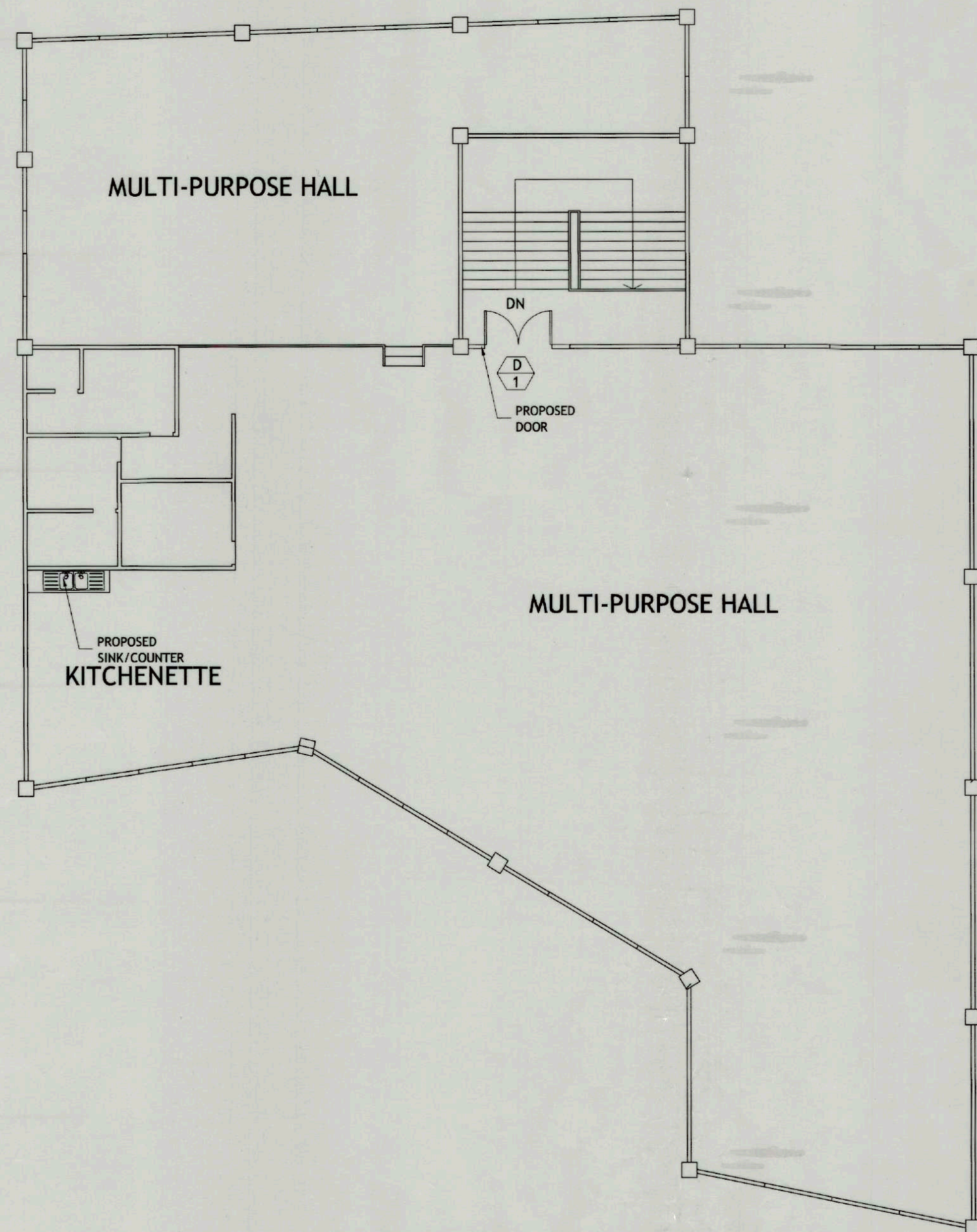
ROOF DECK FLOOR PLAN
