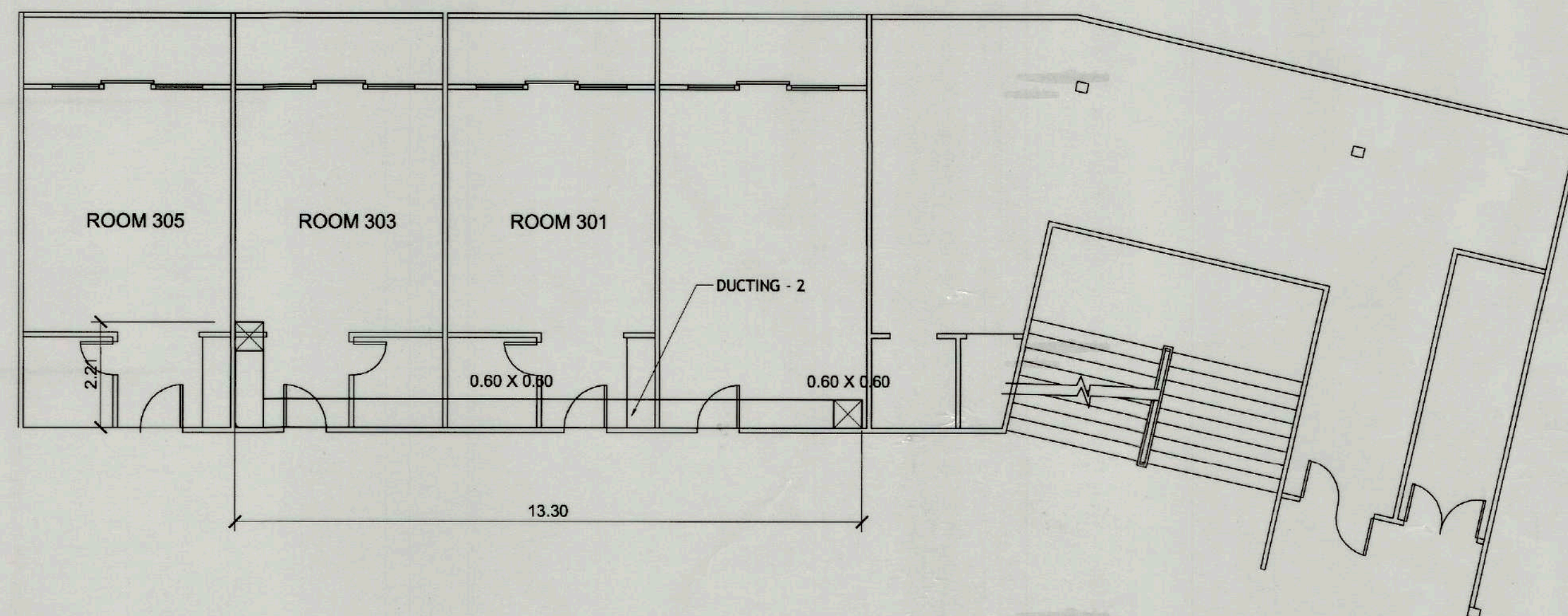
SECOND FLOOR DUCTING LAYOUT NEW BLDG. (PROPOSED)
