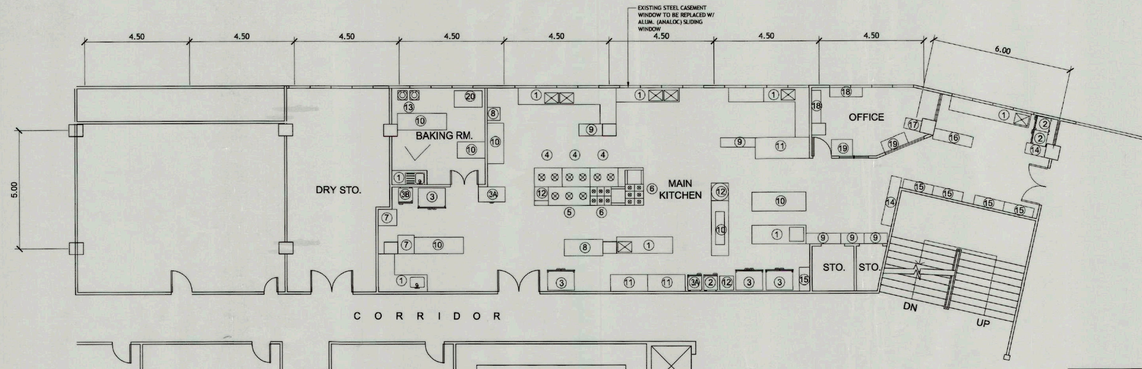
KITCHEN FLOOR PLAN (EXISTING)
