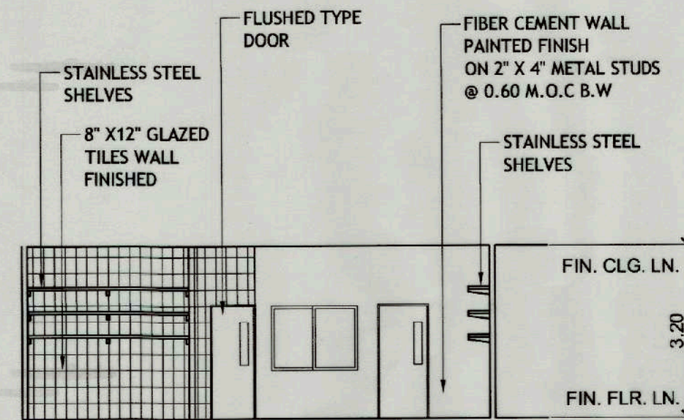
SECTION THRU LINE - D
