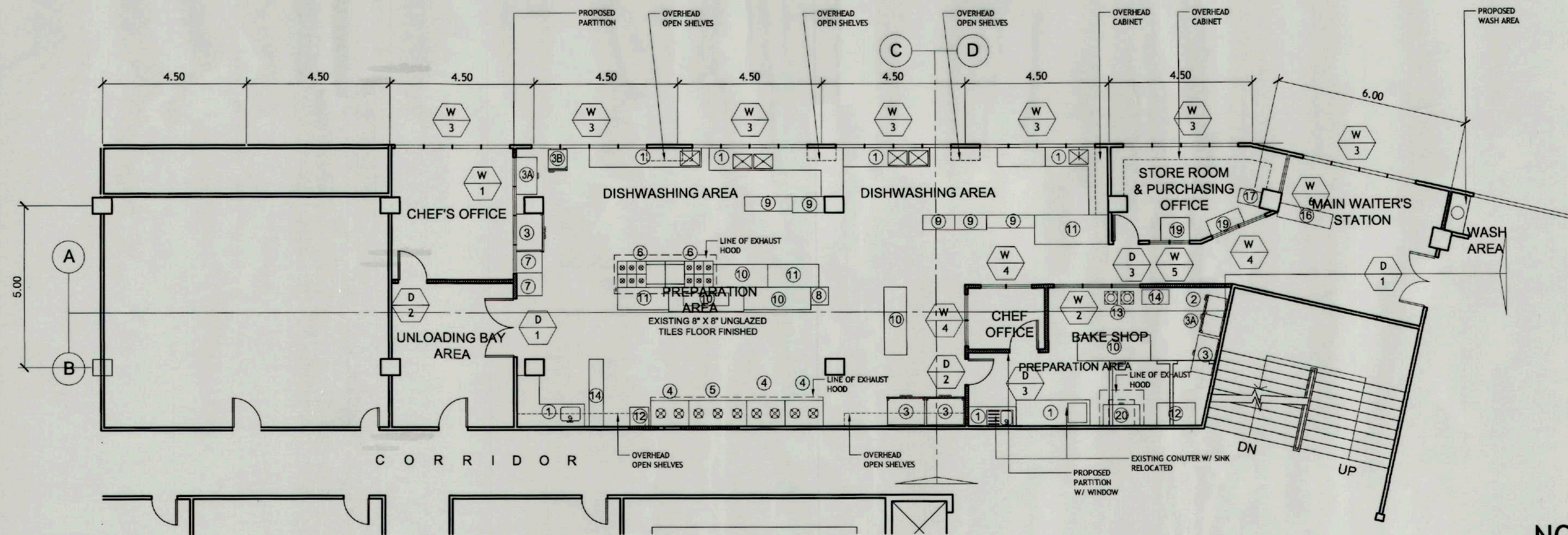
KITCHEN FLOOR PLAN (PROPOSED)
