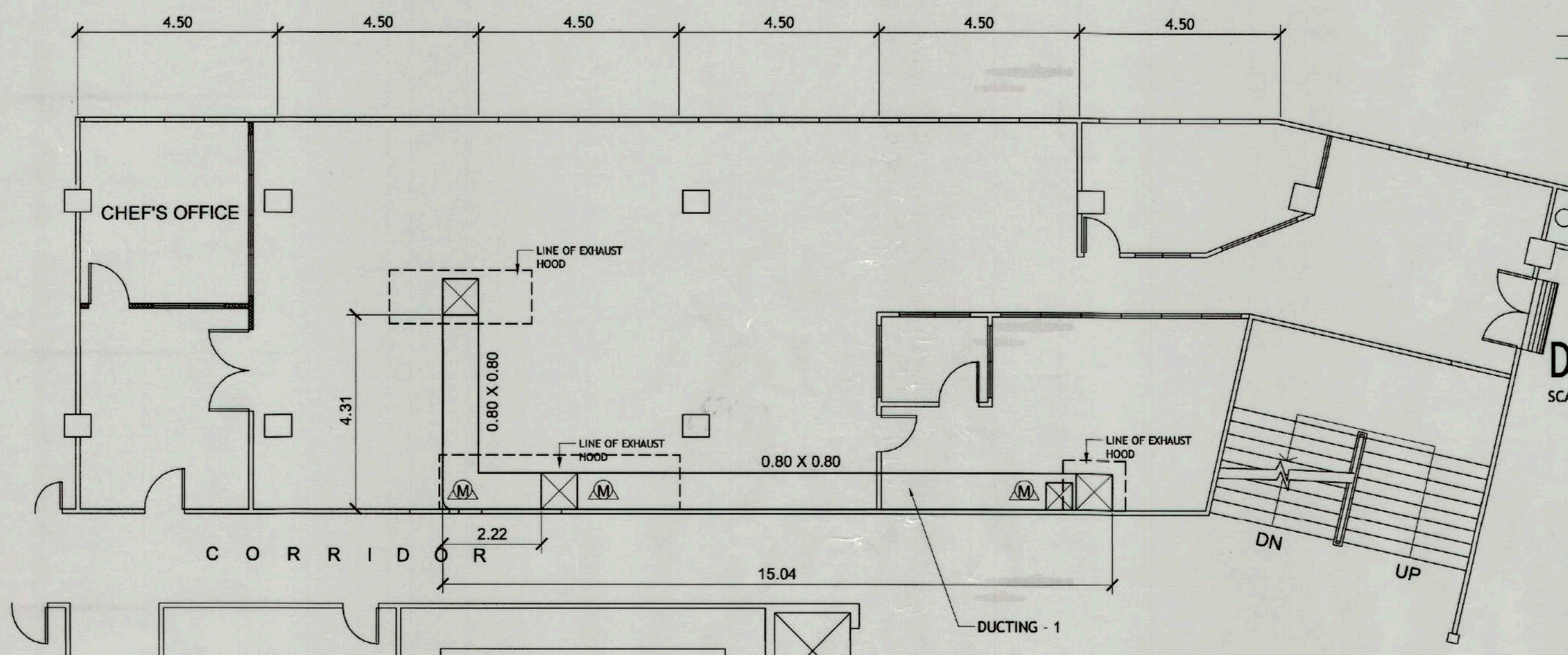
KITCHEN DUCTING LAYOUT (PROPOSED)
