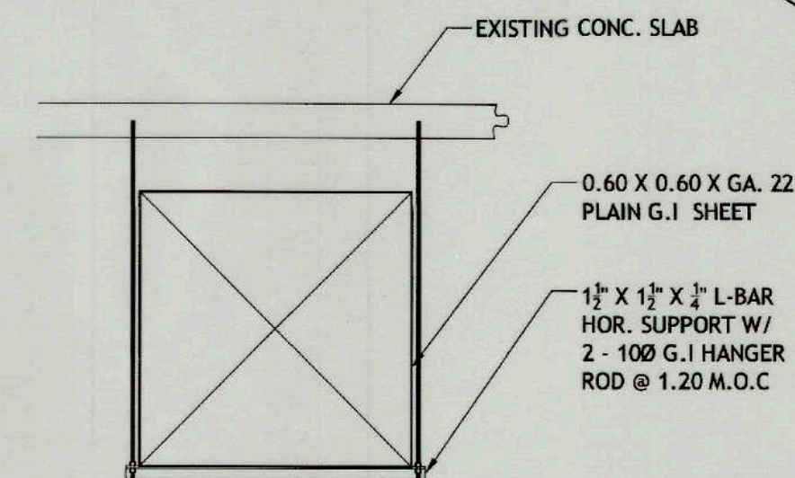
DUCTING - 1 SECTION
