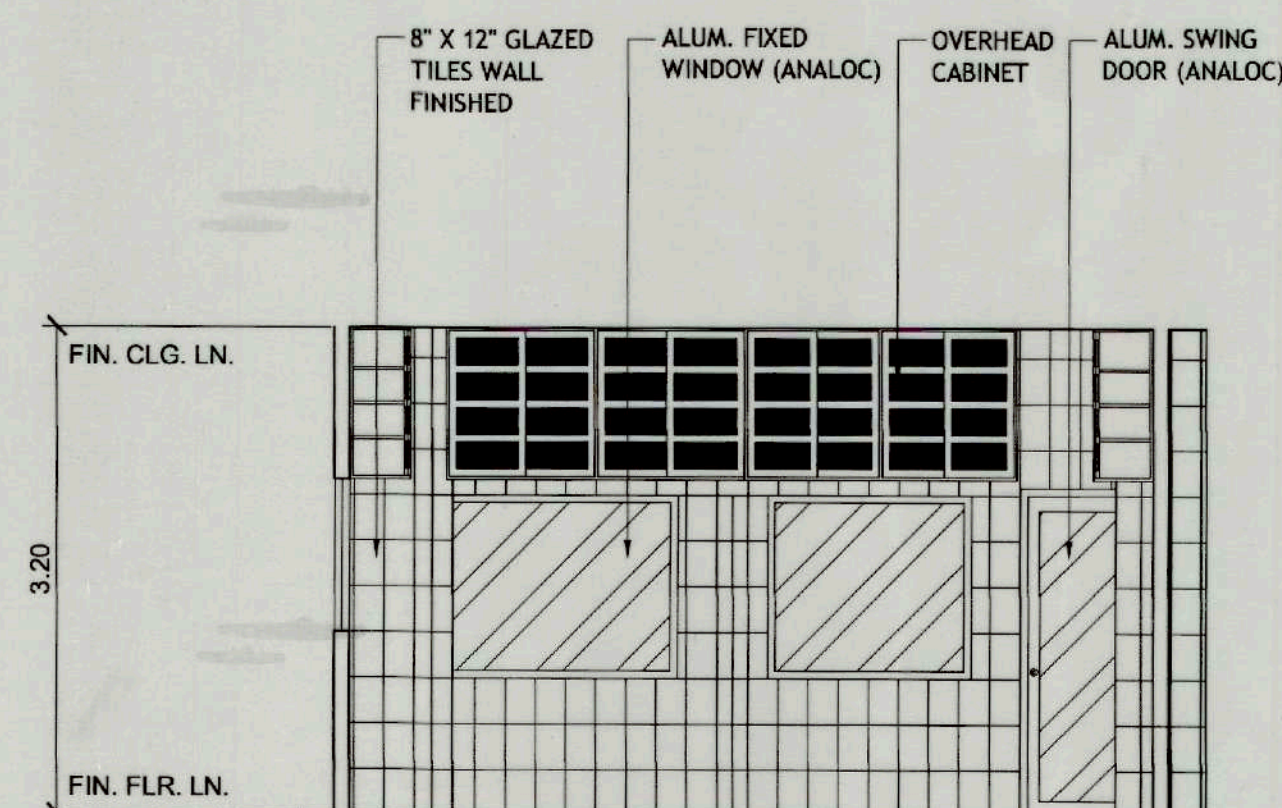
SECTION THRU LINE - B SCALE 1 : 50 MTS
