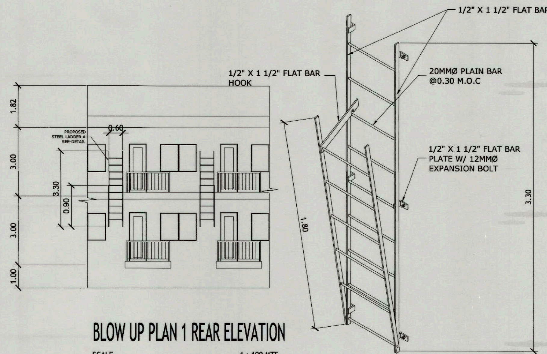
FIRE EXIT LADDER - A DETAIL NOT TO SCALE
