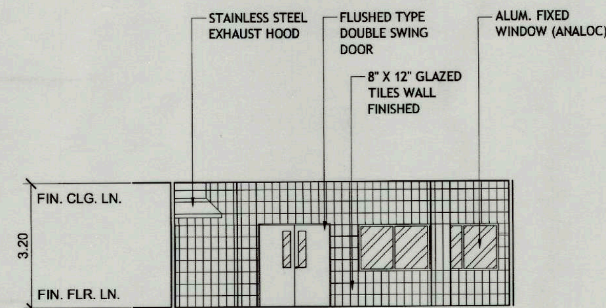
SECTION THRU LINE - C
