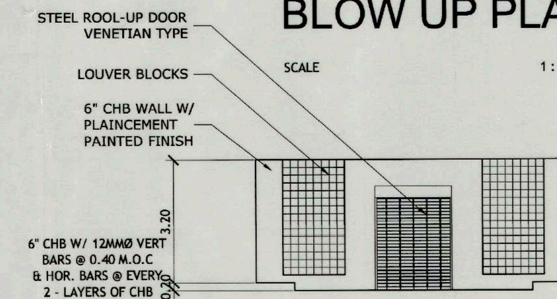
FRONT ELEVATION
