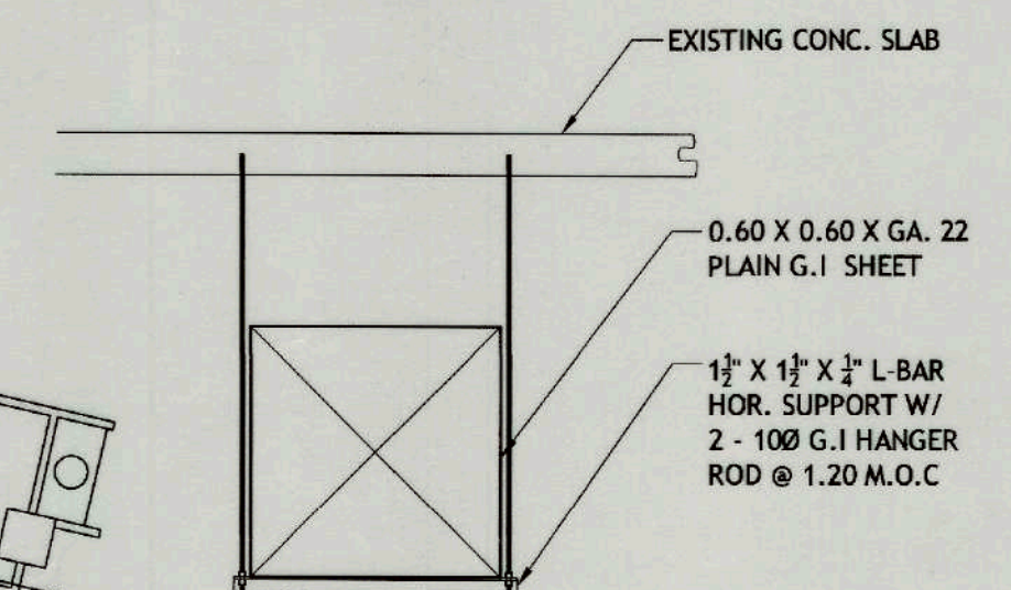
DUCTING - 2 SECTION
