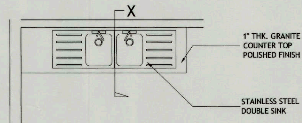
KITCHEN SINK COUNTER PLAN
