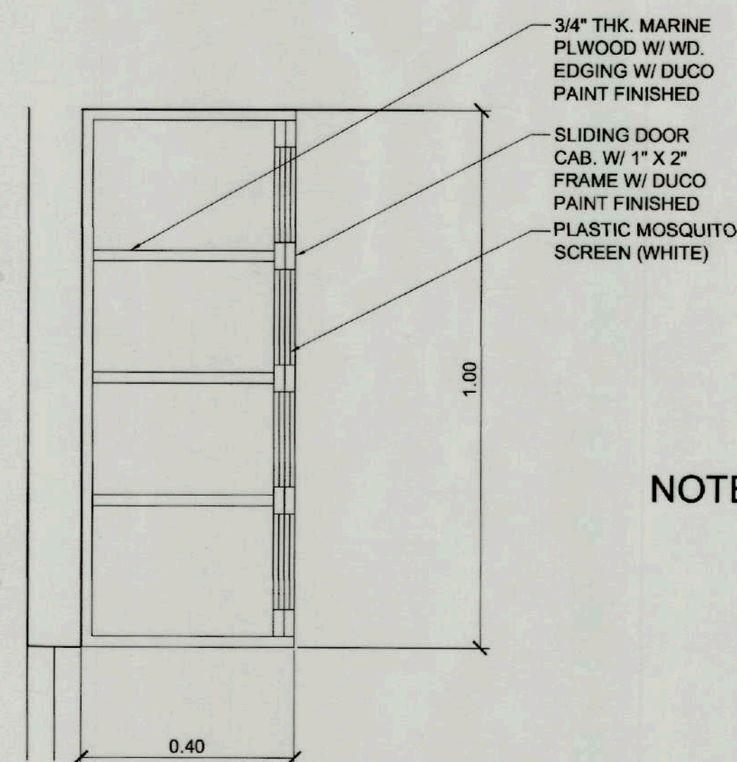
CABINET SECTION SCALE 1 : 10 MTS
