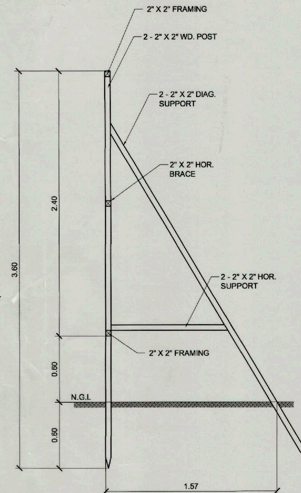
SECTION
