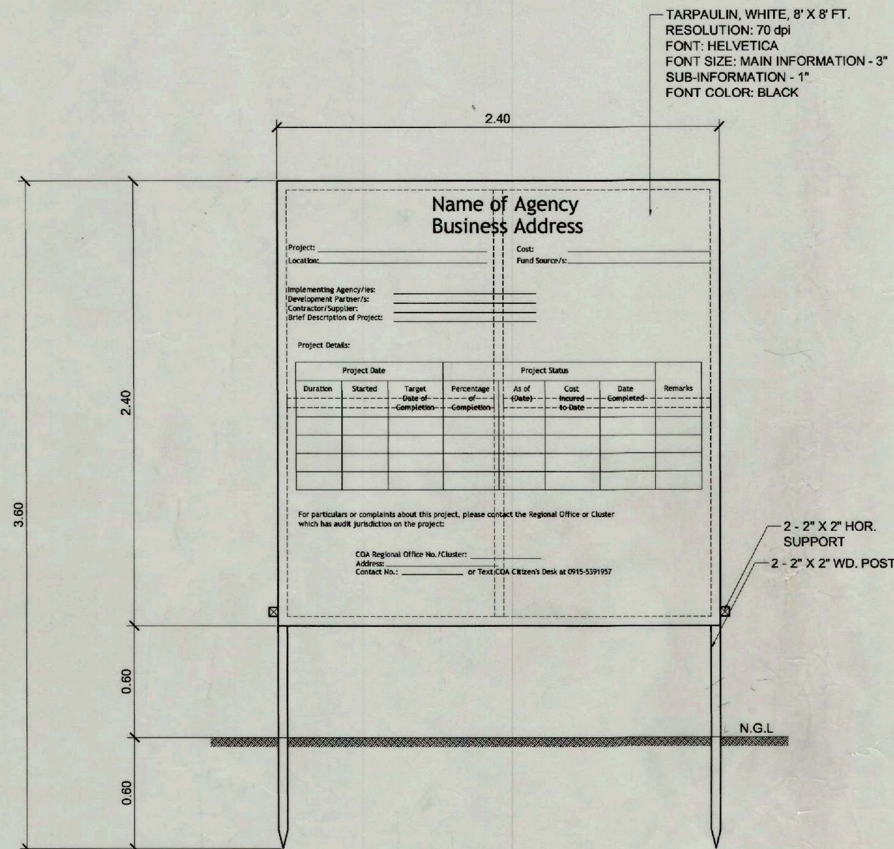
FRONT ELEVATION
