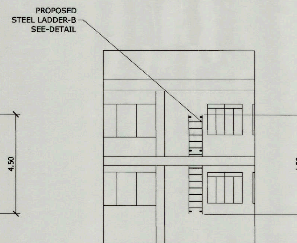
BLOW UP PLAN 3 FRONT ELEVATION SCALE 1 : 100 MTS.
