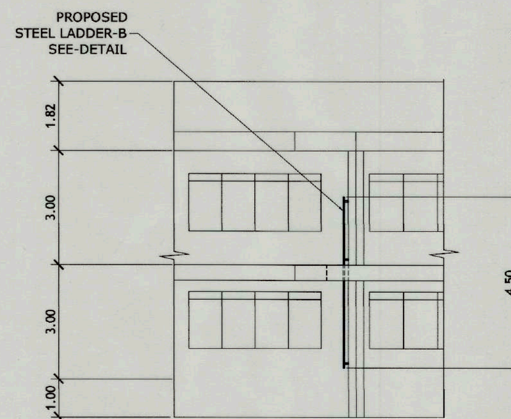
BLOW UP PLAN 2 FRONT ELEVATION SCALE 1 : 100 MTS.
