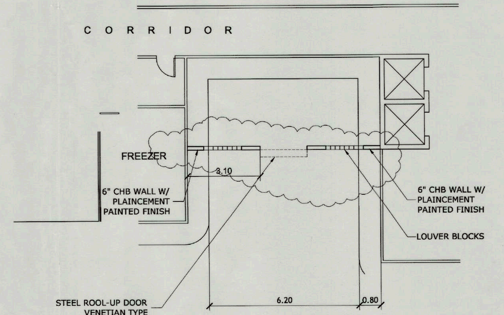
BLOW UP PLAN
