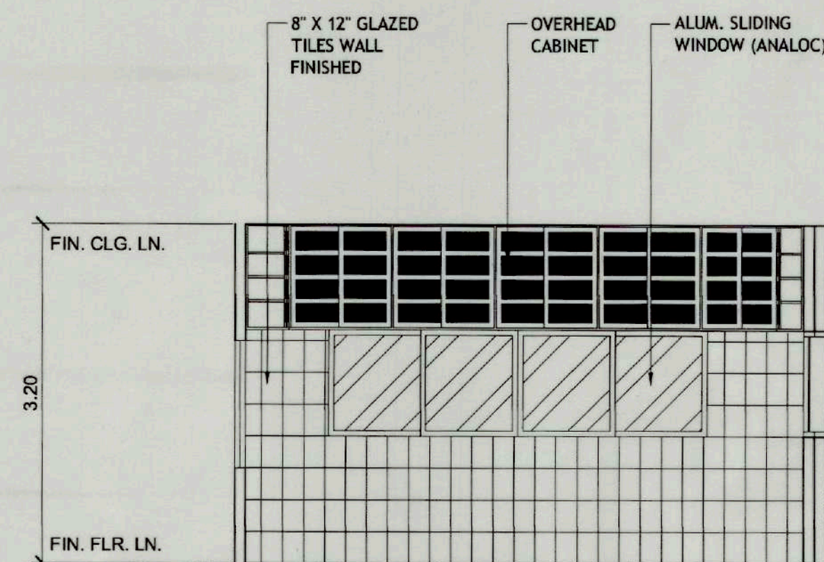
SECTION THRU LINE - A SCALE 1 : 50 MTS
