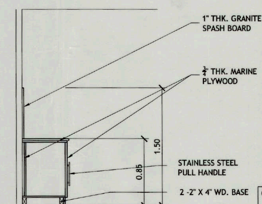
SECTION - X
